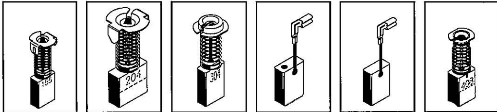
KBMAK155 6.5 x 13.5 x 21/18 mm. AVAILABLE IN STANDARD AND AUTO CUT-OFF KBMAK204 7 x 18 x 18/16 mm. AVAILABLE IN STANDARD AND AUTO CUT-OFF KBMAK304 5 x 11 x 19/16.8 mm. AVAILABLE IN STANDARD AND AUTO CUT-OFF KBMAK318AC 5 x 11 x 15.7 mm. AVAILABLE IN AUTO CUT-OFF ONLY KBMAK325 5 x 11 x 15.8 mm. KBMAK408 6 x 9 x 13/12 mm.
