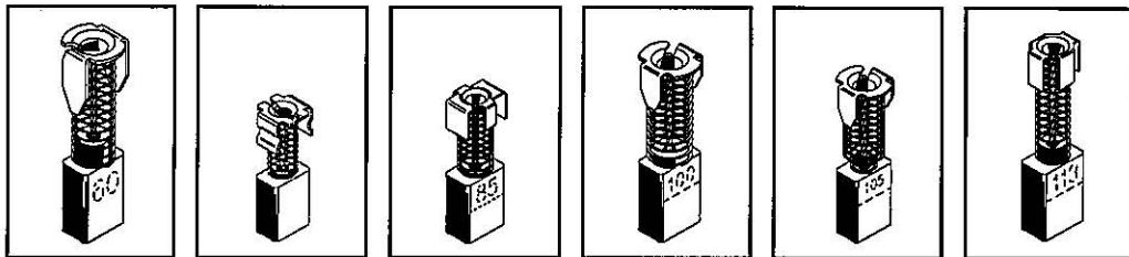
KBMAK60 5 x 8 x 15.5/11.8 mm. KBMAK70A 5 x 8 x 11.9/11 mm. KBMAK85 5 x 8 x 11.5/10.8 mm. KBMAK100 6 x 10 x 16.5/14.8 mm. KBMAK105 6 x 10 x 15 mm. AVAILABLE IN STANDARD AND AUTO CUT-OFF KBMAK113 6 x 10 x 17.5/14.5 mm. AVAILABLE IN STANDARD AND AUTO CUT-OFF
