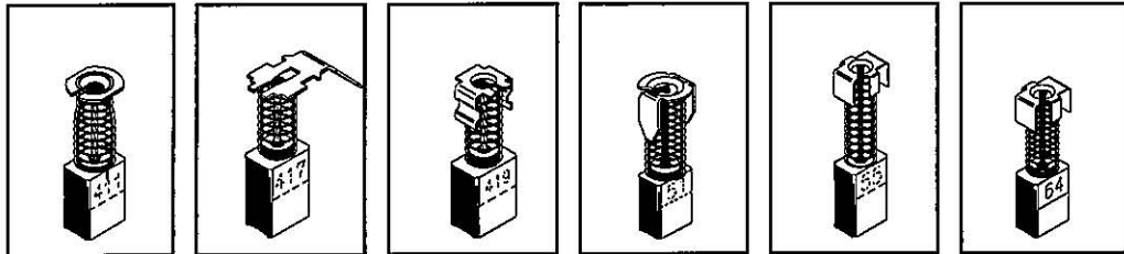
KBMAK410 6 x 9 x 13/12 mm. AVAILABLE IN STANDARD AND AUTO CUT-OFF KBMAK417 6 x 9 x 14.5/13 mm. KBMAK419 6 x 9 x 13.5/11.5 mm. KBMAK51 5 x 8 x 13.5/12 mm. KBMAK55 5 x 8 x 12.5 mm. KBMAK64 5 x 8 x 11.5/10.5 mm.
