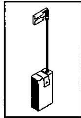
KBBOS122 6.3 x 12.5 x 22 mm.
