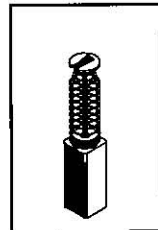
KBBOS507 2(3.15 x 14.1 x 19.7/16.7) mm.
